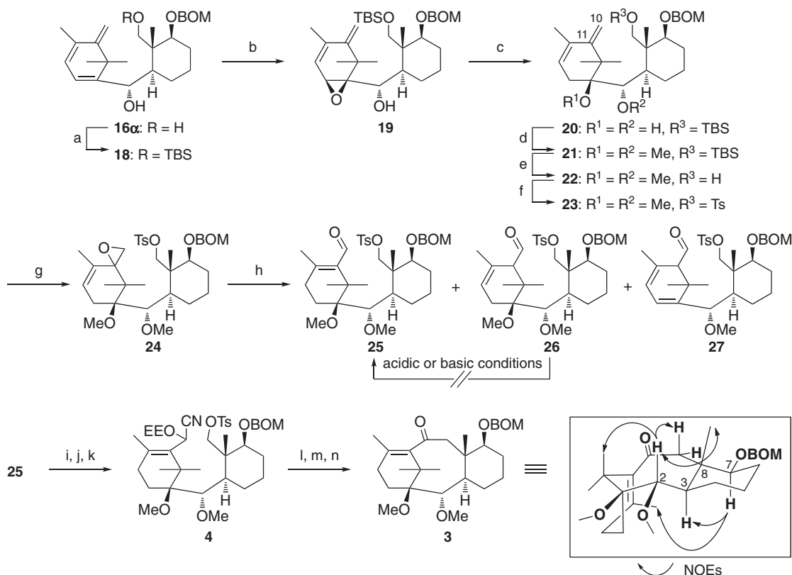
Scheme 5. Construction of the ABC ring 3 . (a) \text{TBSCl} , imidazole, \text{CH}_2\text{Cl}_2 , quant; (b) \text{VO}(\text{acac})_2 , TBHP, benzene, 4^\circ\text{C} ; (c) \text{LiAlH}_4 , \text{Et}_2\text{O} , 0^\circ\text{C} ; (d) \text{NaH} , \text{MeI} , THF; (e) TBAF, THF; (f) \text{TsCl} , DMAP, \Delta , 5 steps 31%; (g) dimethyldioxirane, \text{CH}_2\text{Cl}_2 , 72%; (h) p -TsOH, benzene, 75% ( 25 : 26 : 27 = 4:3:3); (i) \text{TMSCN} , \text{KCN}\cdot\text{DC-18-Cr-6} ; (j) \text{HCl} , THF; (k) EVE, CSA, \text{CH}_2\text{Cl}_2 , 0^\circ\text{C} , 3 steps 83%; (l) \text{LiN}(\text{TMS})_2 dioxane, \Delta , 43%; (m) CSA, MeOH; (n) \text{NaOH} , \text{Et}_2\text{O} , 2 steps 42%.
