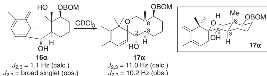
Scheme 4. Stereochemical assignment of the 2-OH group in 17 \alpha .
