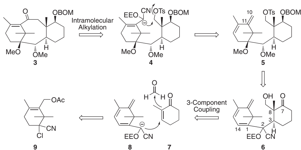
Scheme 1. Synthetic strategy for the ABC ring system of taxanes.
