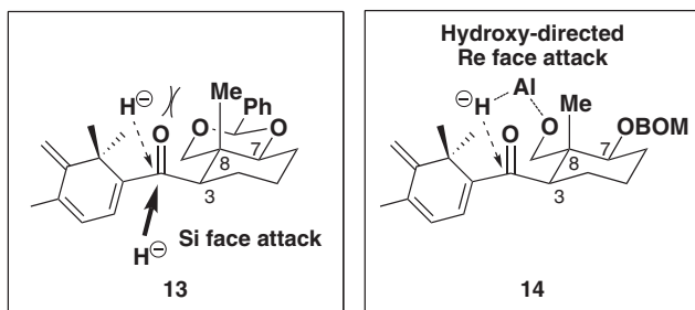
Figure 2. Proposed mechanism in the stereoselective reduction of the ketones 13 and 14 .
