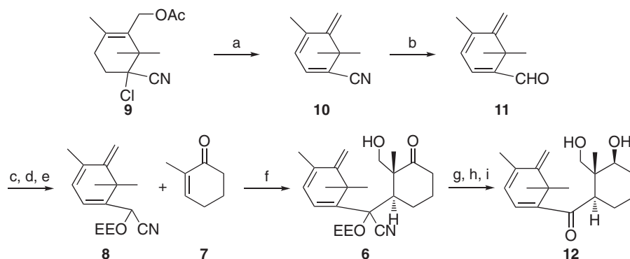
Scheme 2. Preparation of the AC ring 12 . (a) DBU, benzene, reflux, quant; (b) i -Bu 2 AlH, toluene, -78^{\circ}\text{C} , quant; (c) TMSCN, KCN·DC-18-Cr-6; (d) 1 M HCl, THF; (e) EVE, CSA, CH 2 Cl 2 , 0^{\circ}\text{C} , 3 steps 95%; (f) i -Pr 2 NLi, THF then HCHO, -78^{\circ}\text{C} , 90%; (g) NaBH 4 , MeOH; (h) CuSO 4 , MeOH/H 2 O; (i) 1 M NaOH aq. Et 2 O, 3 steps 61%.
